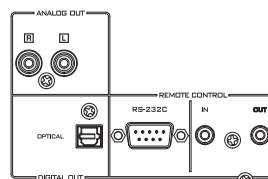
CD-C600RK Rear Panel
