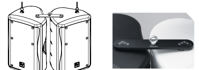
CB5 CLUSTER BRACKET KIT
