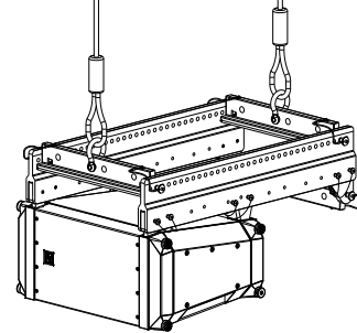
X12TC-GRID PULL-UP KIT
