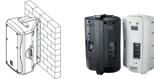
ZX3 and ZX5 MB3 or MB5 WALL/CEILING MOUNT BRACKET
