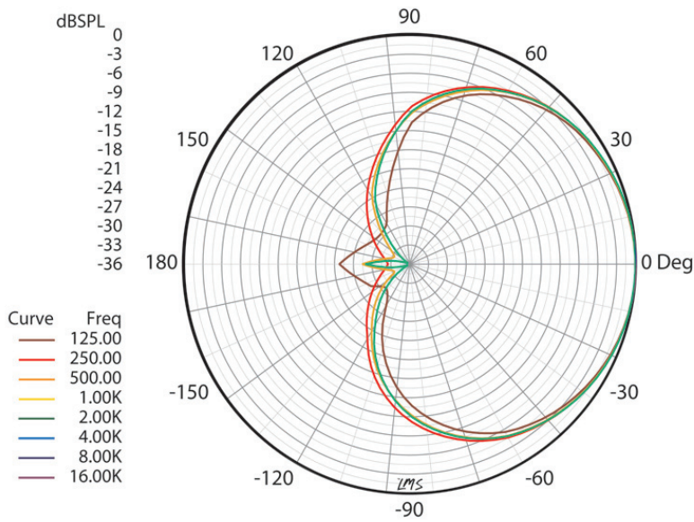
Cardioid 125 Hz - 1K
