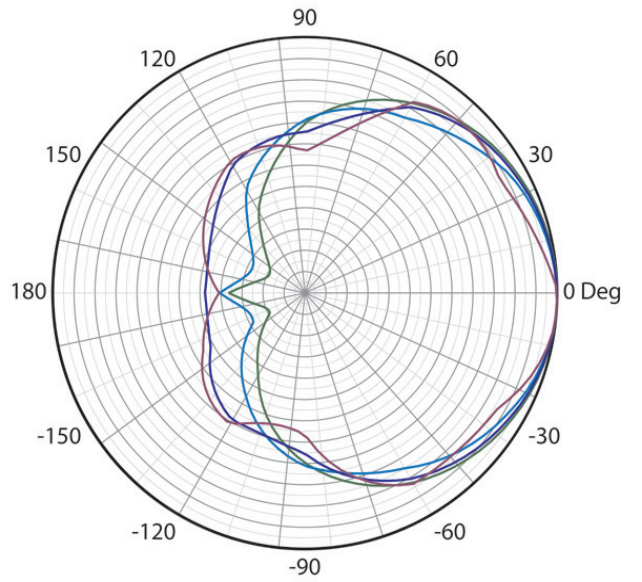
Cardioid 2 K - 16 K
