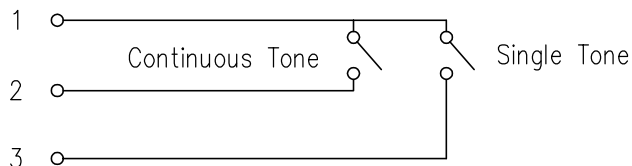
Connection Diagram
