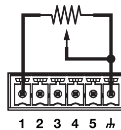
Example: GPI connections for a potentiometer
