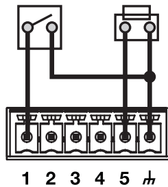
Example: GPI connections for switches
