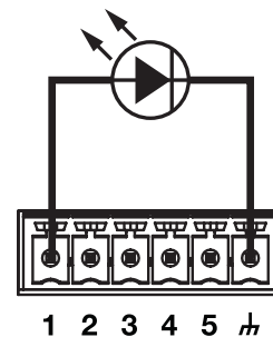
Example: GPO connections for a current sink
