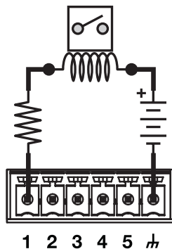
Example: GPO connections for a current source
