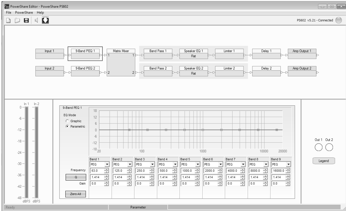
Figure 10. PowerShare Editor software 2-channel configuration for PS602 and PS602P amplifiers
