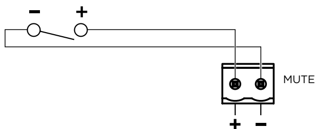
Figure 6. Amplifier mute contact closure
