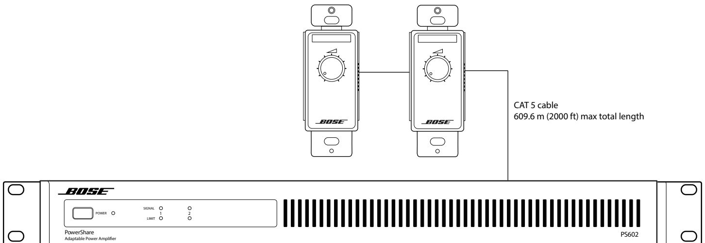
Figure 8. Direct CC-1 ControlCenter zone controller connection to amplifier
