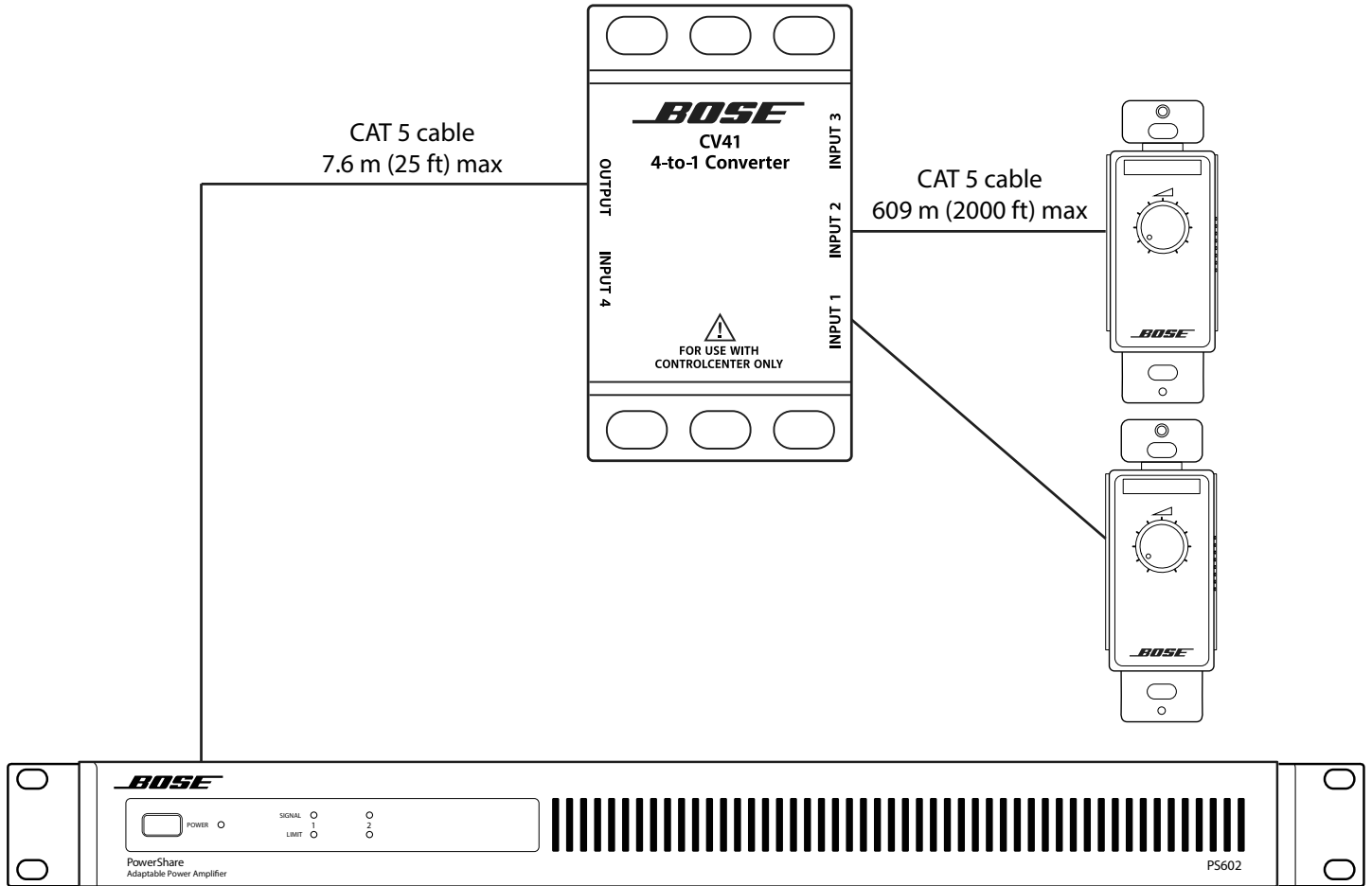
Figure 9. Distributed CC-1 ControlCenter zone controller connection to amplifier
