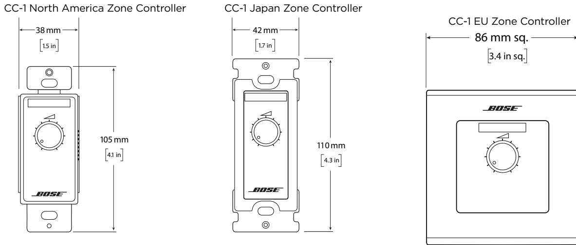
Figure 7. CC-1 ControlCenter zone controllers
