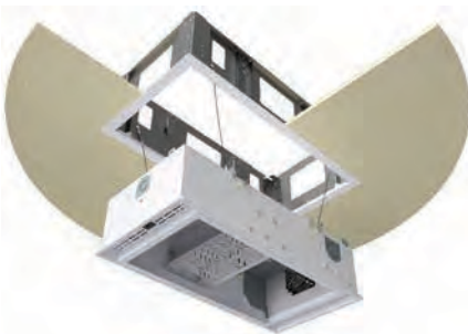
CB-SR12 with CB-12 (shown in service position)
