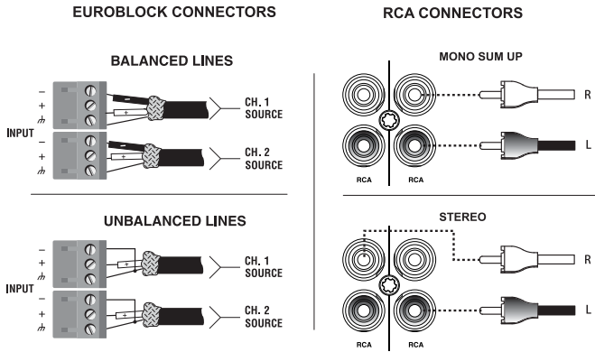
Figure 2.4 Input Wiring
