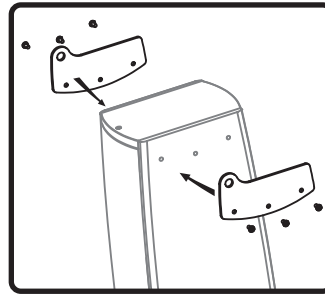
3. Attach AC-LA8-FLY hanging adapter plate(optional accessory) to left and right sides of speaker using bolts supplied with accessory kit.
