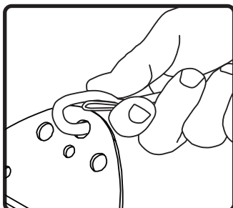
6. Attach included safety cable from bent bracket to secure mounting point on structure. Installer to supply structural fastener.
