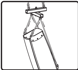
5. Attach speaker to One-Way-Array bracket using Allen Products flying hardware. Cables should connect to hanging adapter plates at the top, and back plate near the bottom of the cabinet.
