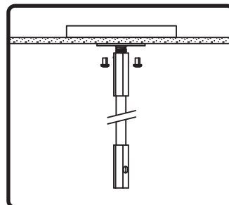
4. Attach Allen Products MM-020x mounting plate/pole (available separately) to ceiling. Use hardware with sufficient strength to reliably hold the speaker.
