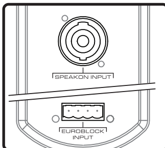
7. Choose one of two inputs: SpeakOn,™ or included Euroblock. Note: If using LA808i, refer to wiring instructions 7-11.
