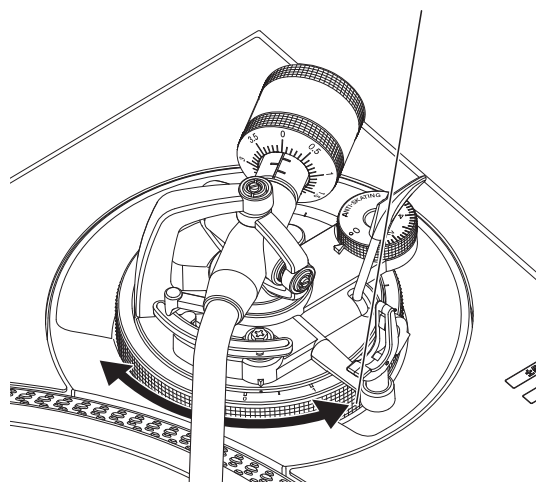
[HEIGHT ADJUST]-Drehrad
