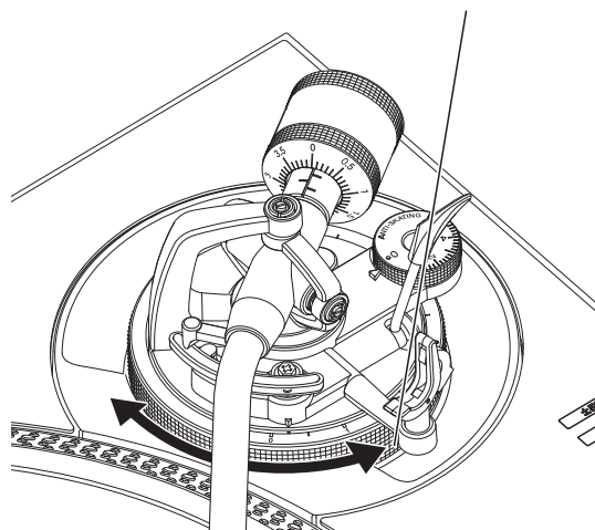
Dial de [HEIGHT ADJUST]
