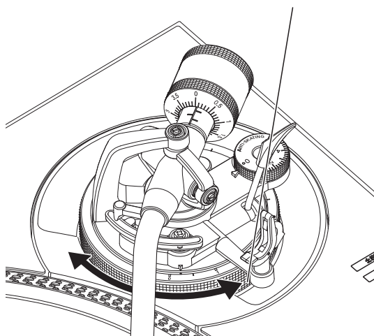
Molette [HEIGHT ADJUST]
