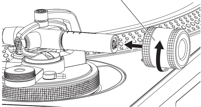
Balance weight
