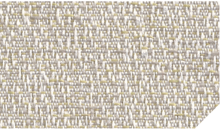
Sandstone
