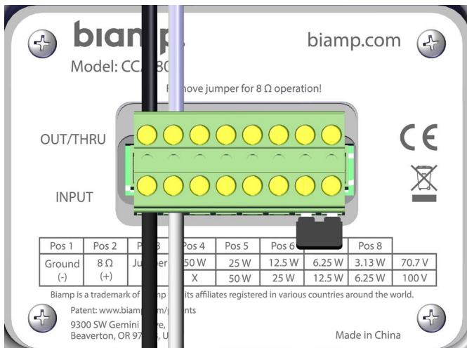
Cabinet with pass-thru connection (8 Ω operation shown)
