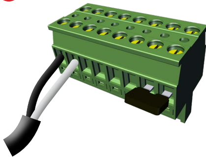
Low Impedance operation (move preinstalled jumper to unused terminals)
