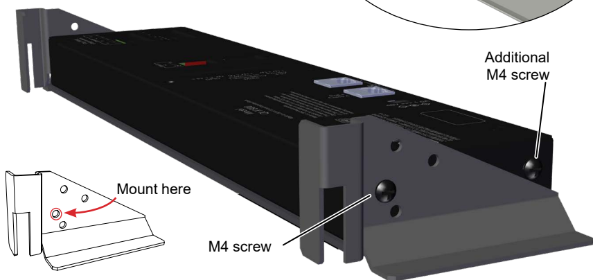
Figure 38. Controller is face down against the ceiling tile with an additional M4 screw on each side to prevent panel movement
