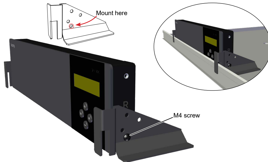
Figure 39. Base of controller is flush with the bottom of the brackets
