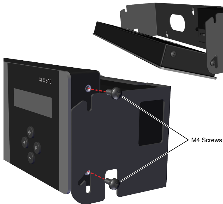
Figure 35. Mount unit to wall bracket and rotate down
