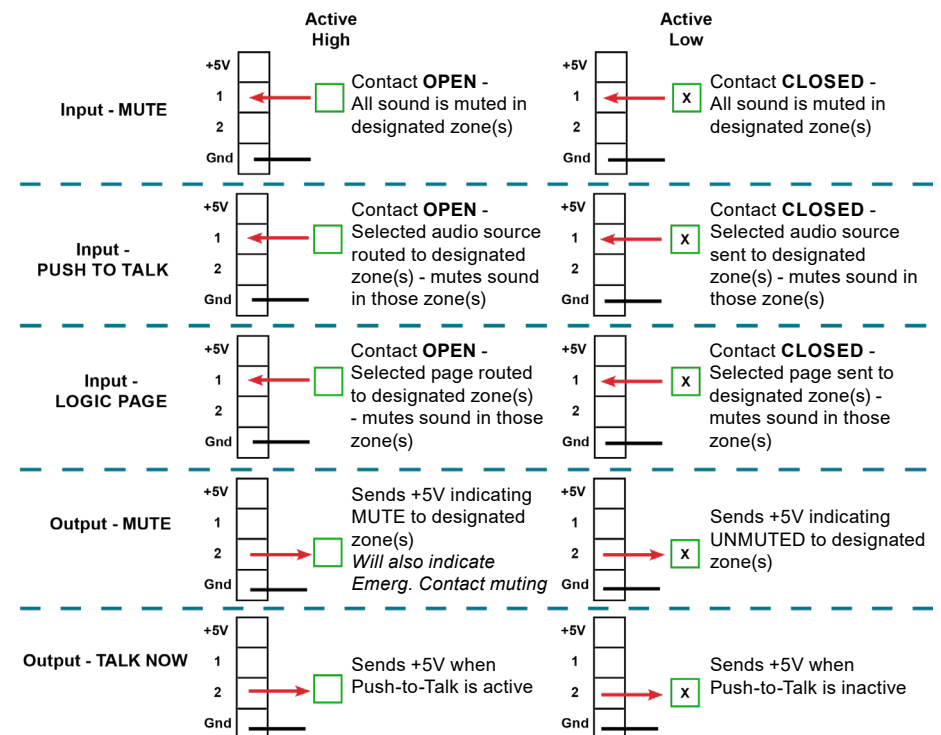
Figure 8. GPIO connection / wiring
