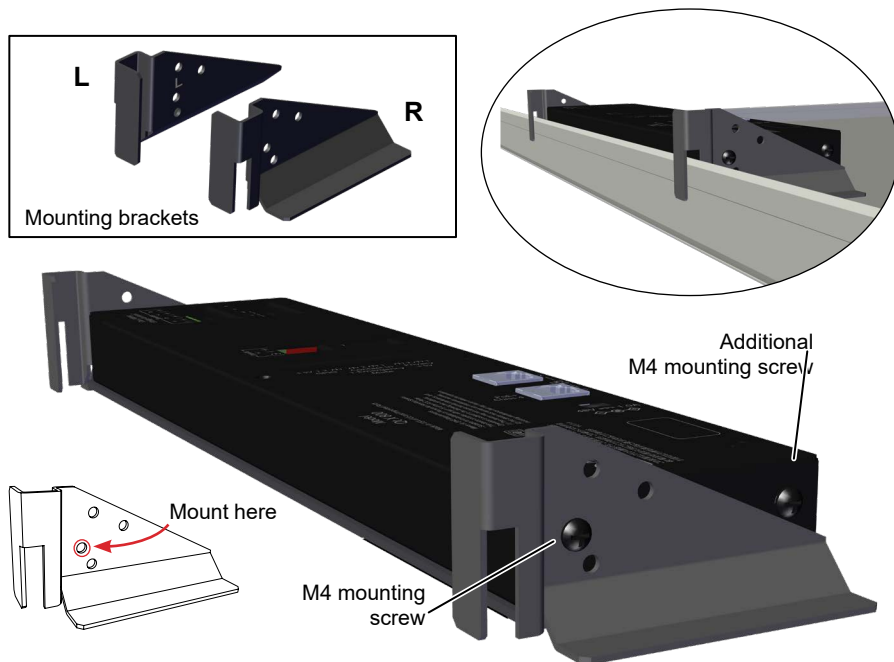
Figure 3. Controller is face down against the ceiling tile Installation Note: An additional M4 screw must be installed in the lower holes on each side to prevent panel movement
