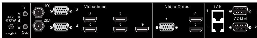
Figure 1-1: Back Panel
