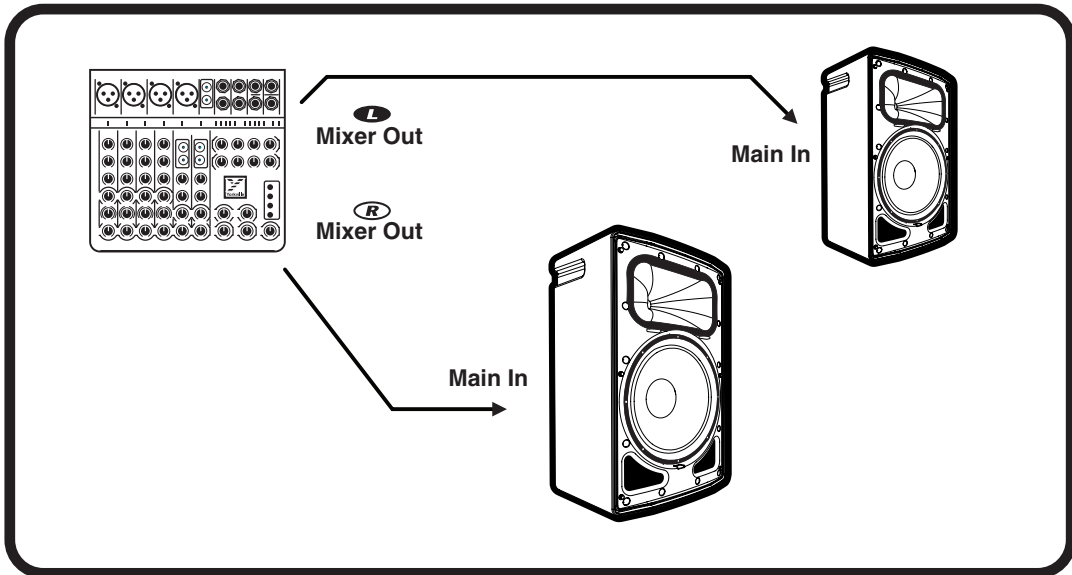
STEREO P.A., with EXTERNAL MIXER
