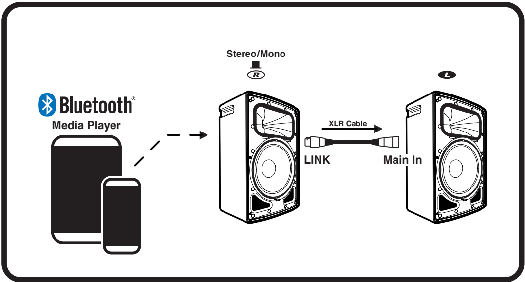
Stereo Operation with Bluetooth® MEDIA PLAYER
