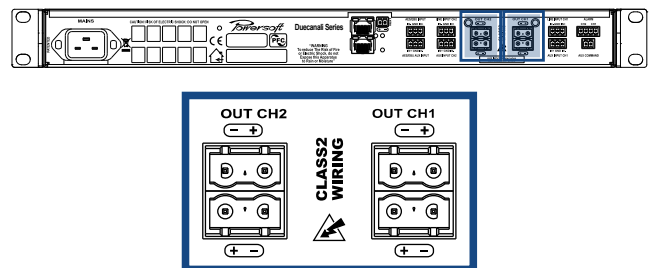
FIGURE 13: Output connectors
