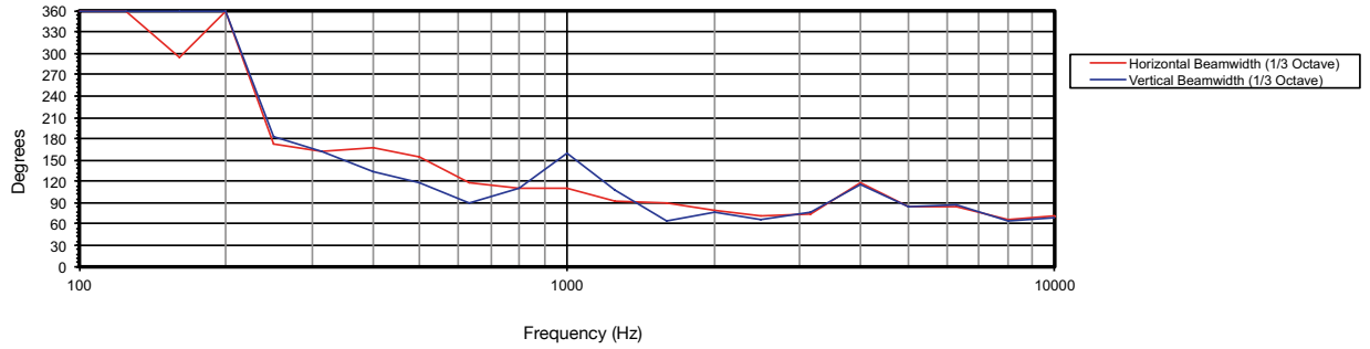
Beamwidth vs Frequency
