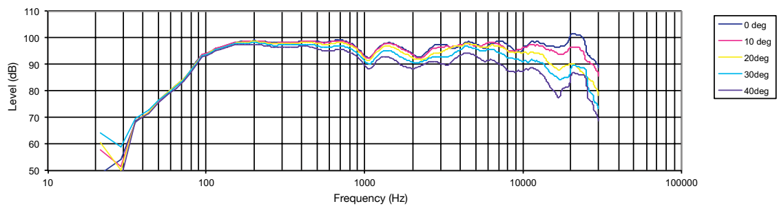
Off-axis Frequency Response
