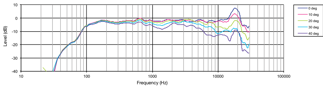
Horizontal off-Axis Response
