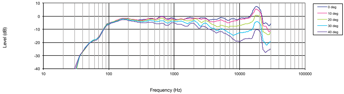
Vertical off-axis Frequency Response
