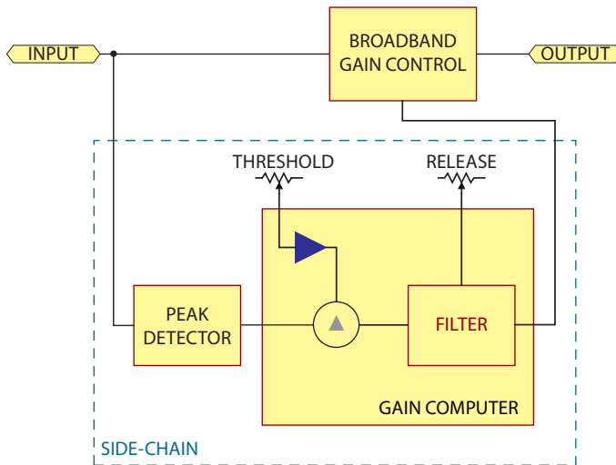
Figure 7. Peak Limiter Block Diagram
