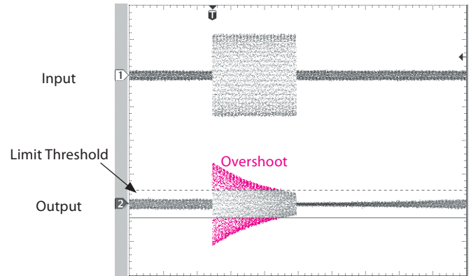
Figure 9. Compressor used as a limiter. Signal peaks can still exceed threshold, even at high ratio settings.
