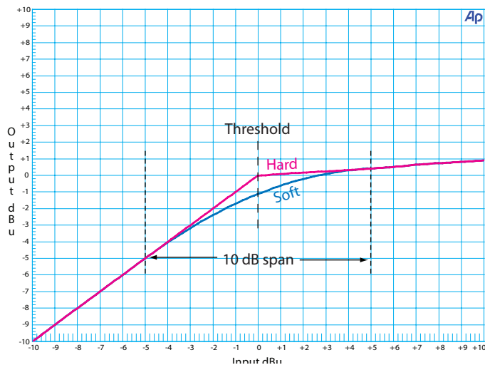
Figure 15. The Hard Knee compression characteristic has a 0 dB span. The Soft Knee compression characteristic has a 10 dB span.
