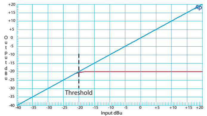
Figure 10. Peak Limiter Response Graph
