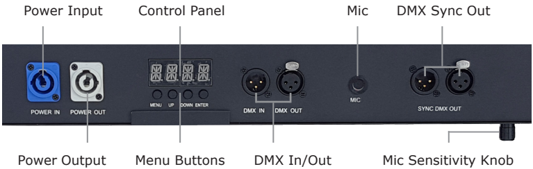
Figure 2: The Rear Connections
