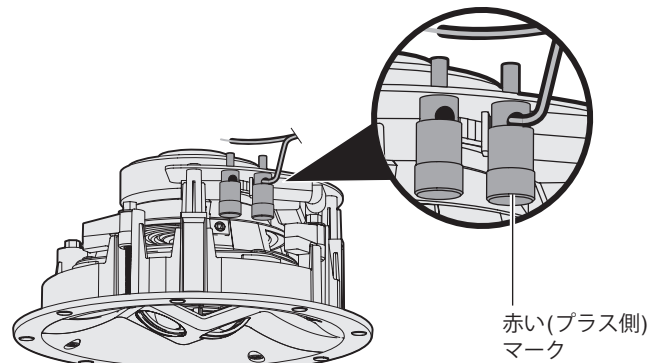
Virtually Invisible® 591 speaker
