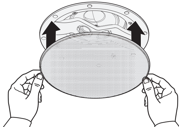
Virtually Invisible® 591 -kaiutin
